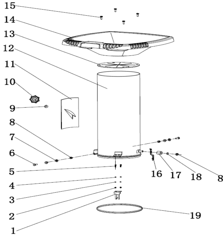
FIG.1 RARO2400E Top intake opening
